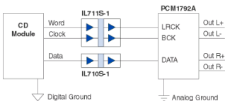
Low-Jitter Isolation
